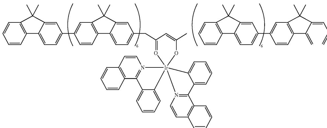
Compound 1
