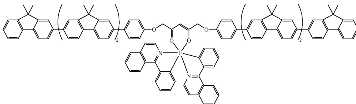
Compound 2
