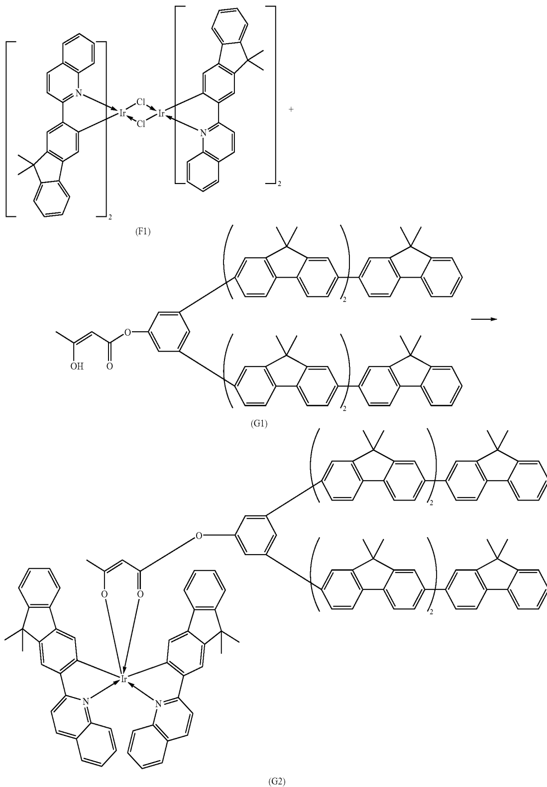
Synthesis Scheme G
