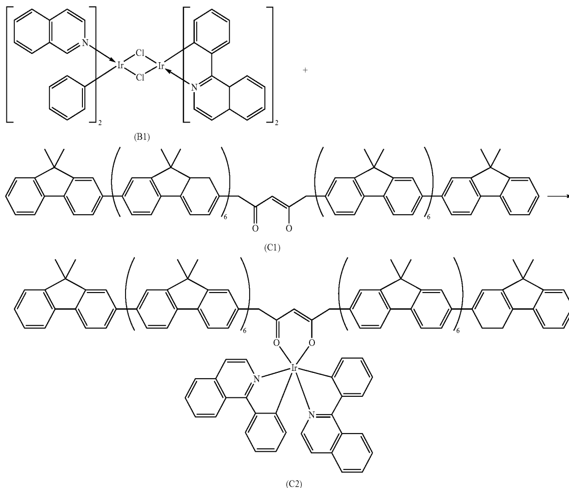
Synthesis Scheme C
