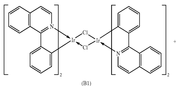
Synthesis Scheme D
