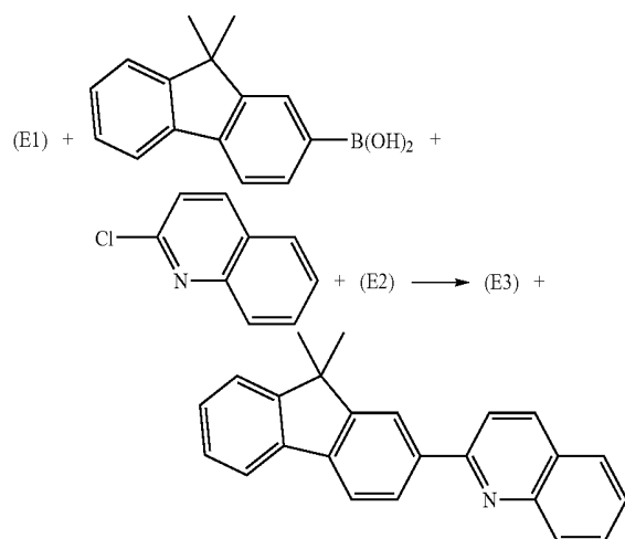
Synthesis Scheme E
