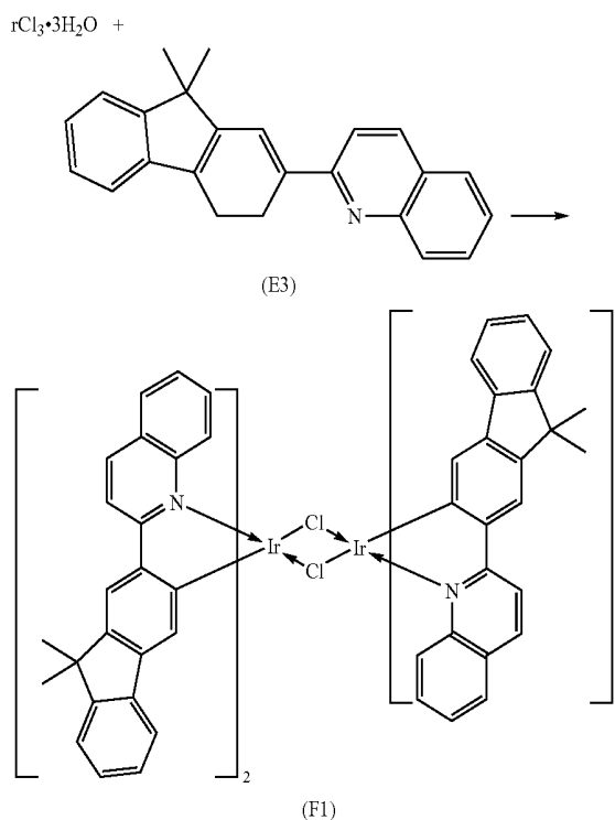
Synthesis Scheme F
